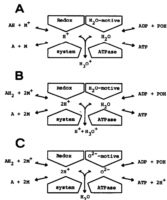
Fig.7. Microscopic chemiosmotic coupling mechanisms: (A) Protonic anhydride mechanism with protonic exit pathway specific for H 3 O + uniport or H + -H 2 O symport. (B) as (A) but with protonic exit pathway specific for 2H + -H 2 O symport. (C) Miniaturisation of macroscopic chemiosmotic mechanism.
